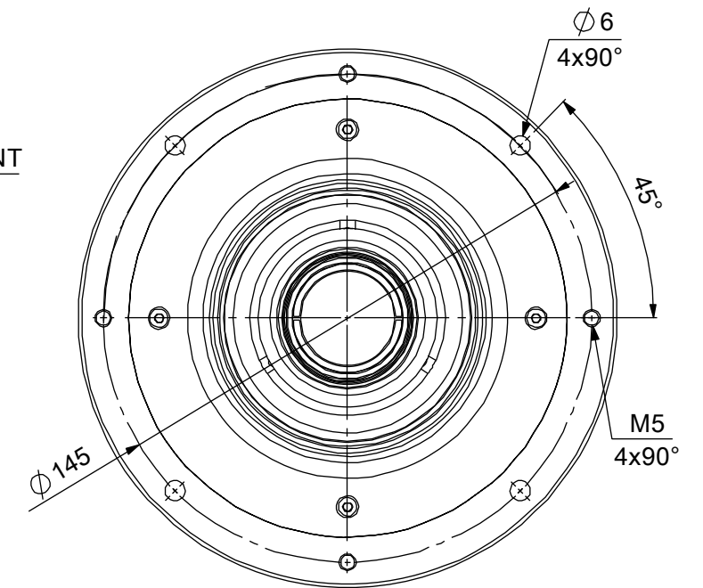
MOUNTING PORTION DETAIL VIEW フランジ取付部詳細
